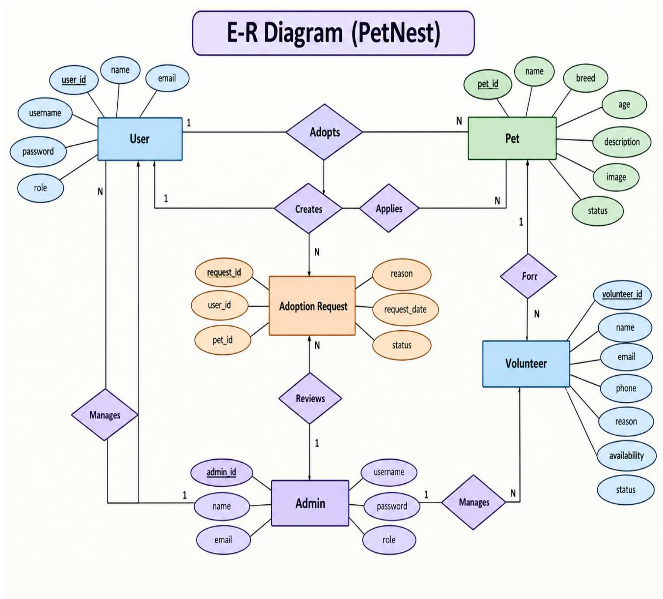
Entity-Relationship Overview
