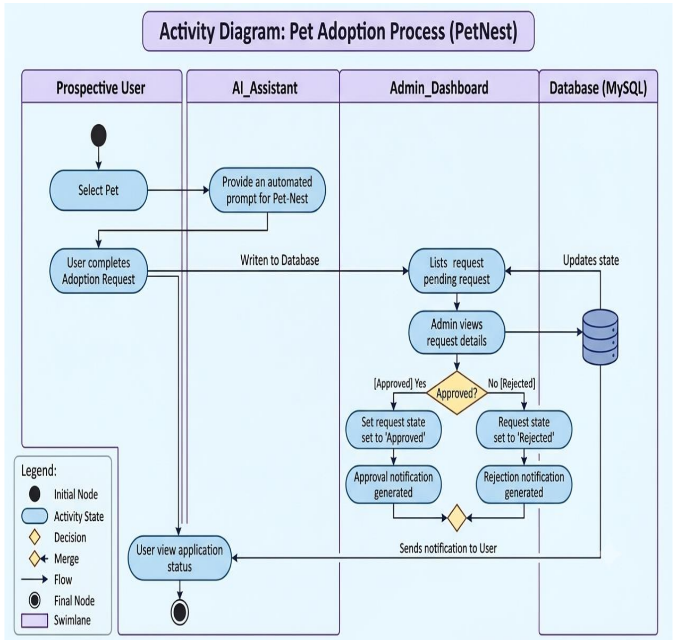
Pet Adoption Activity Diagram
