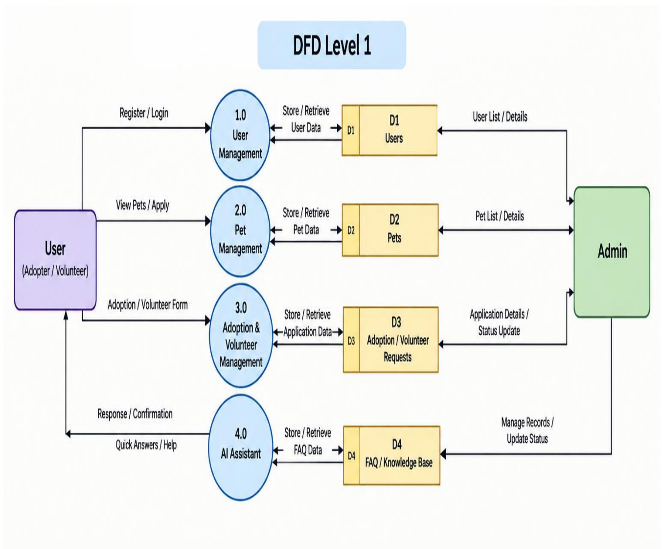
Level-1 Data Flow Diagram
