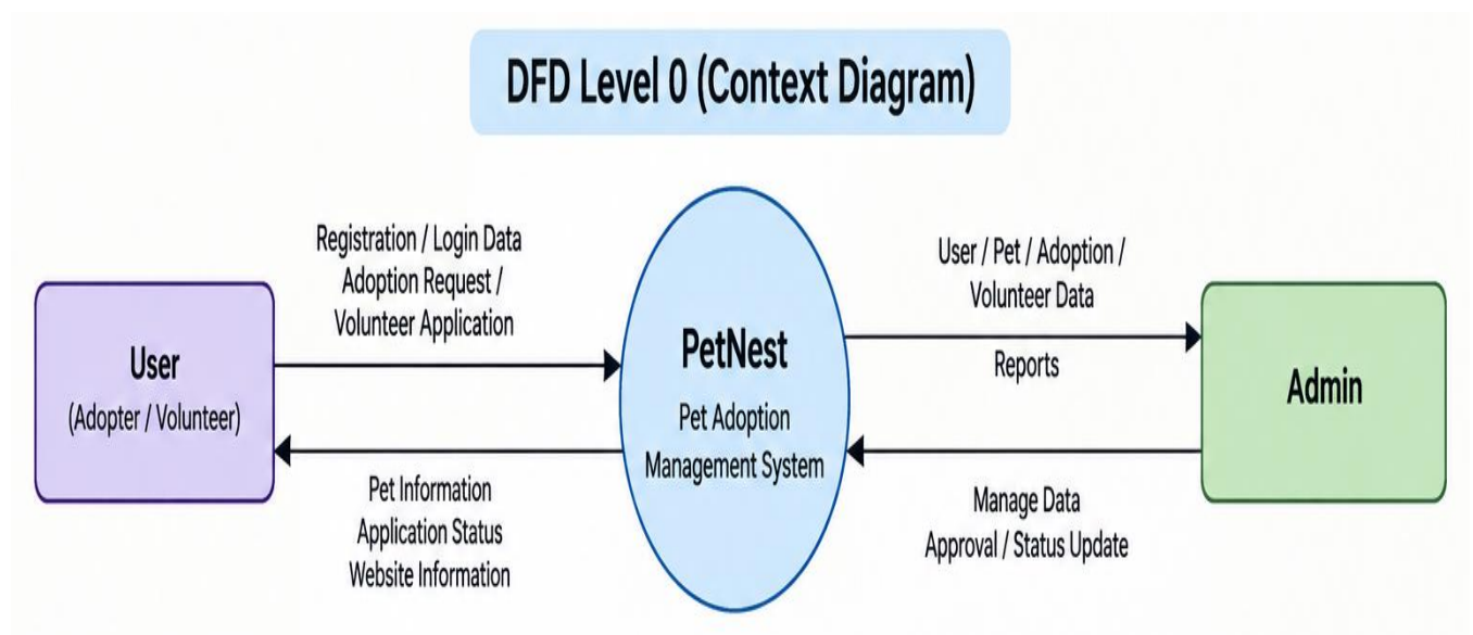
Level-0 Data Flow Diagram
